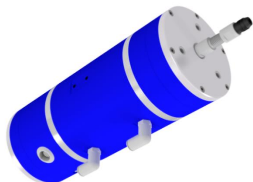
Figure 2: X-Act 325 shaker with collet and stinger for modal testing
